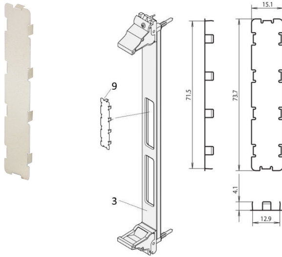
04610028 Item 9: EMC cover; Item 3: front panel
