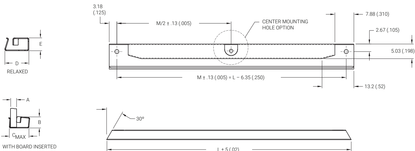
FLARED ENTRY OPTION DETAIL
