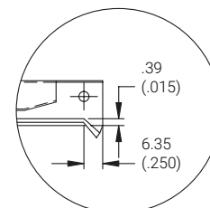
FLARED ENTRY OPTION DETAIL
