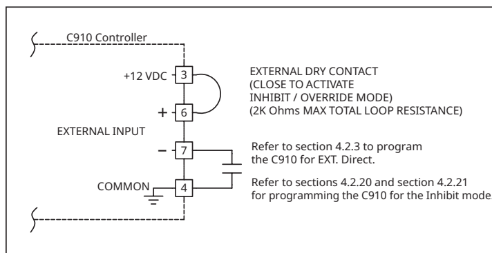
Fig. 2.5 – Wiring for External Device Control/Override
