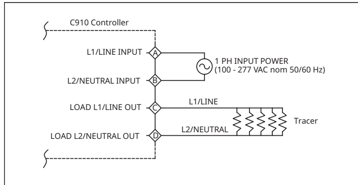
Fig. 2.3 – Power Connection
