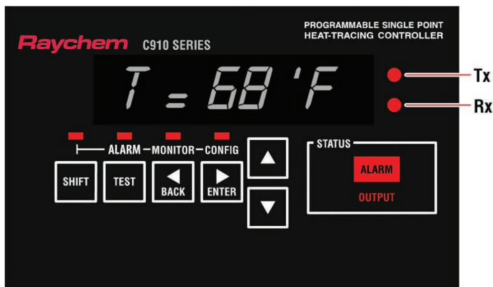
Fig. 3.2 – Operator Console
