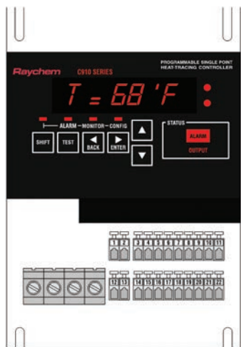
Fig. 2.2 – Power Connection
