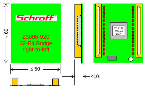
CPCI Rear Brick Bridge 32Bit, right-to-left
