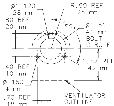
Large Ventilator
