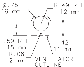
Small Ventilator
