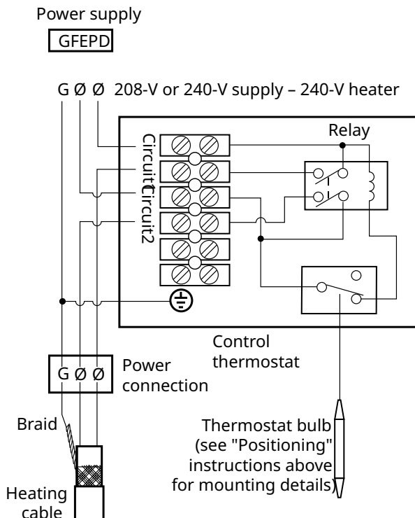
Figure 1. Heat-tracing control
