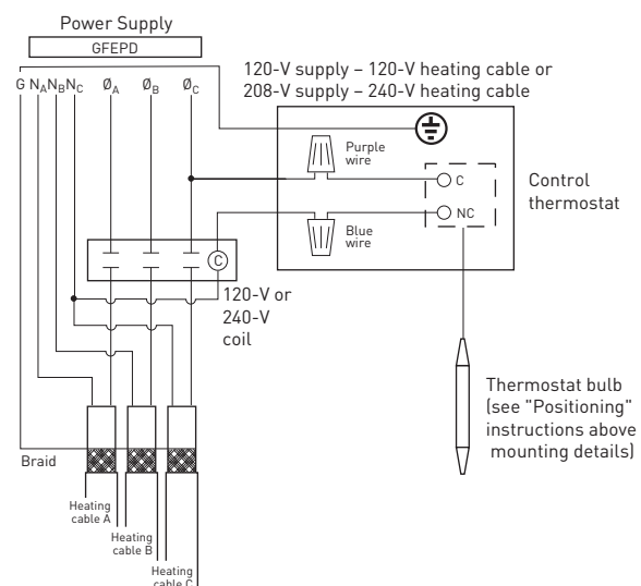
Figure 2. Contactor control
