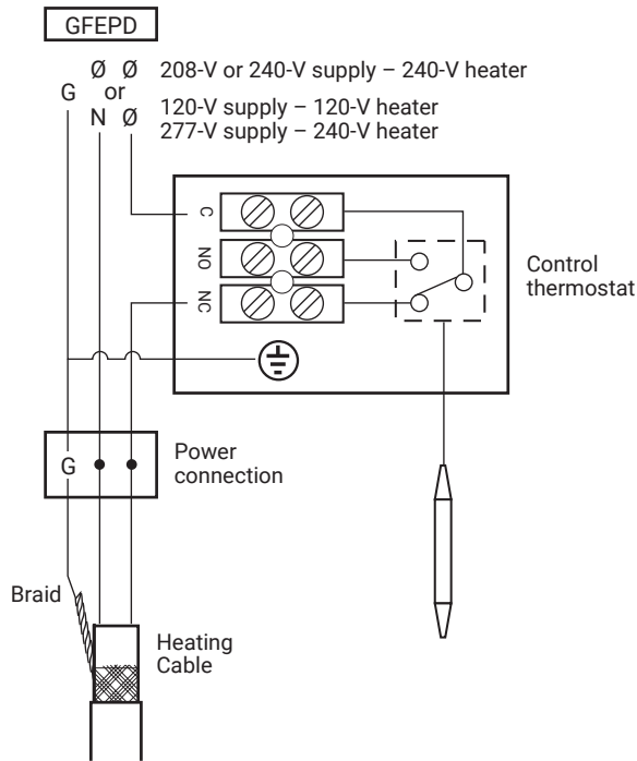
Figure 1. Heat-tracing control
