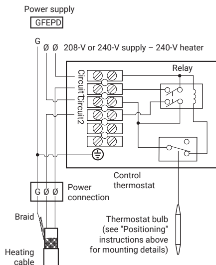
Figure 1. Heat-tracing control
