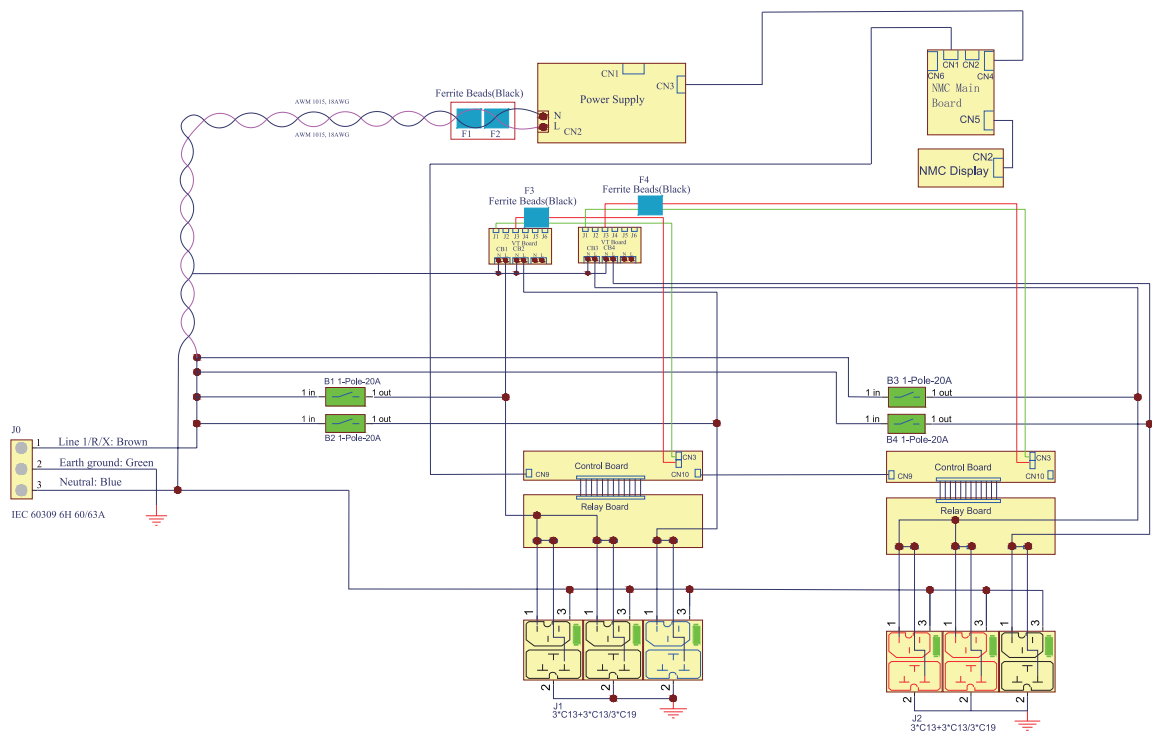
INTERNAL WIRING SCHEMATIC
