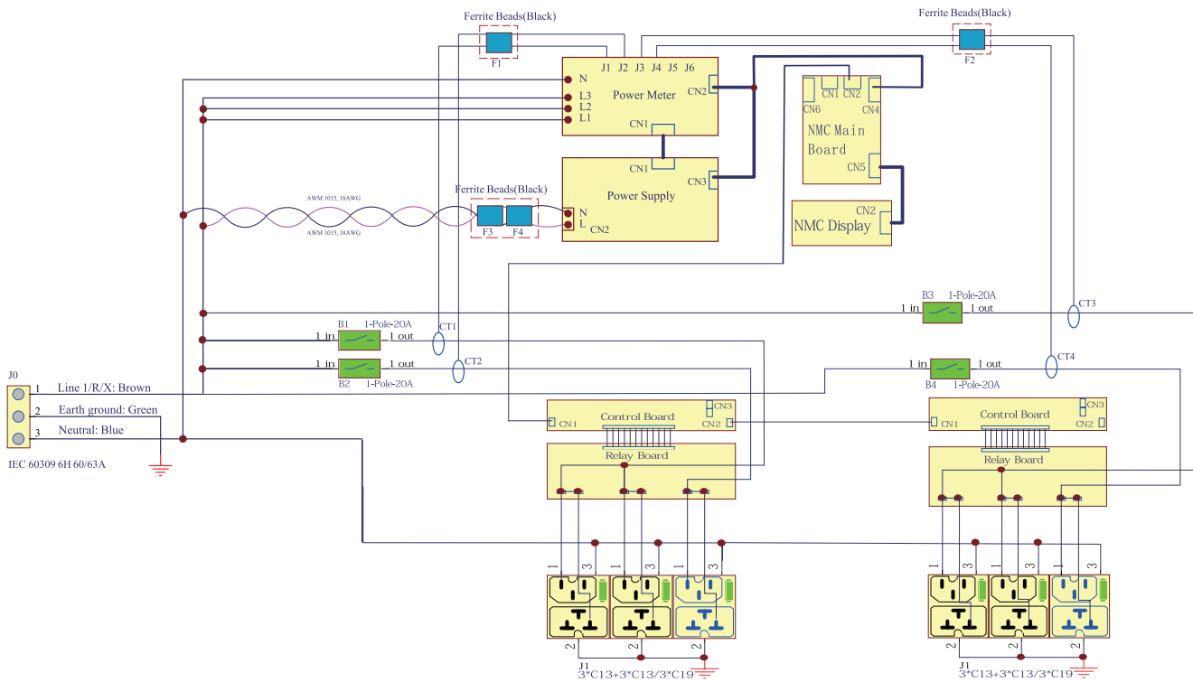
INTERNAL WIRING SCHEMATIC
