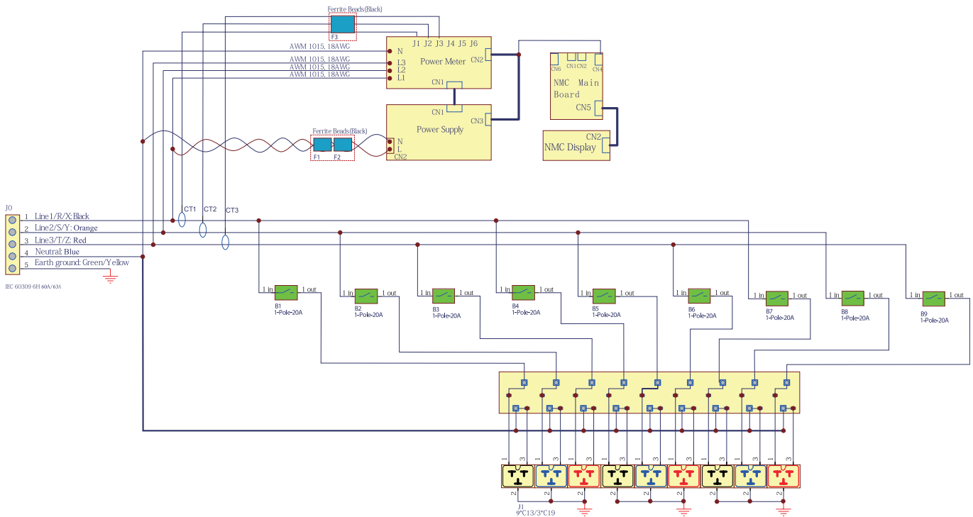
INTERNAL WIRING SCHEMATIC
