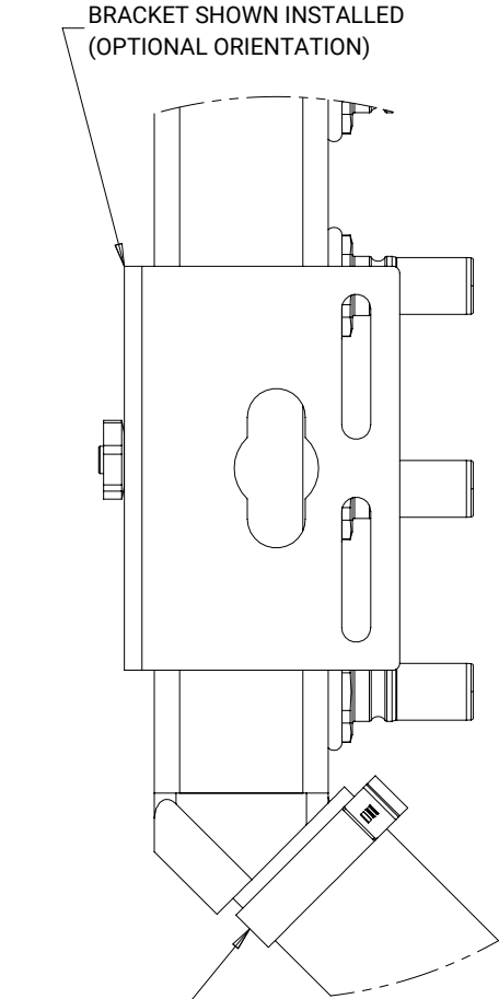
DETAIL B
