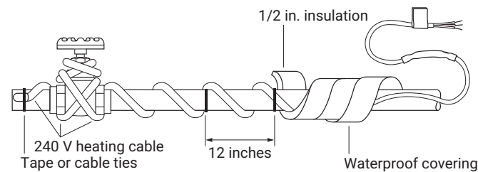
Spiral-traced Installation
