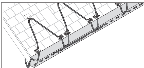
Roof and gutter de-icing: standard roof
