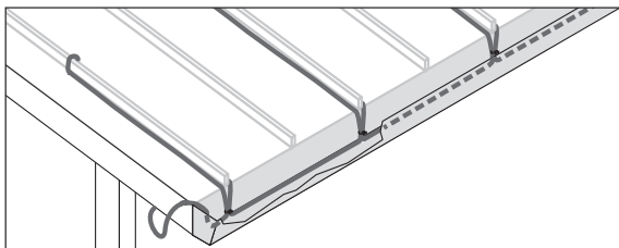
Roof and gutter de-icing: standing seam metal roof
