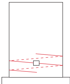
Fig. 3 Heating cable arrangement on a vertical tank
