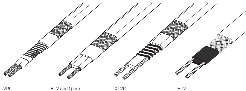
Fig. 1 Self-regulating heating cables
