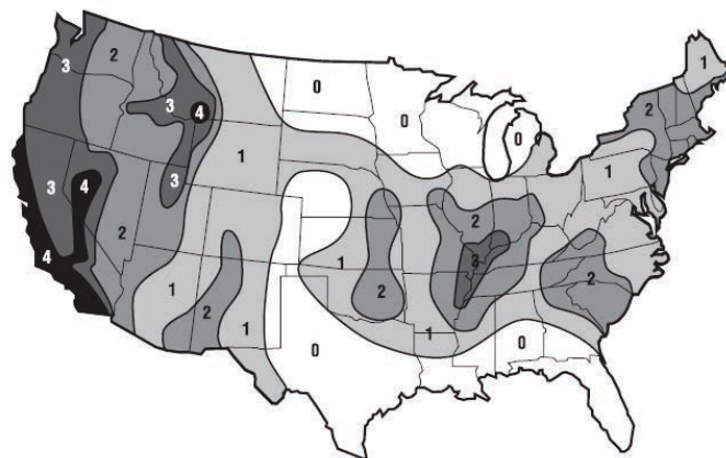
Figure 1. Telcordia Seismic Zones
