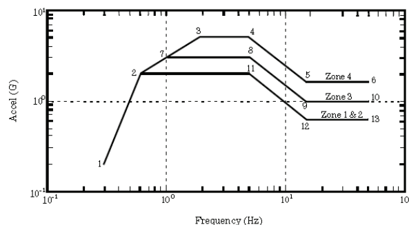
Figure 2. Required Response Spectra
