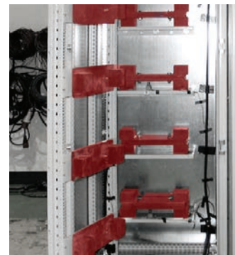
Figure 6. MCS20086R5 Loaded mounting plate and swing frame
