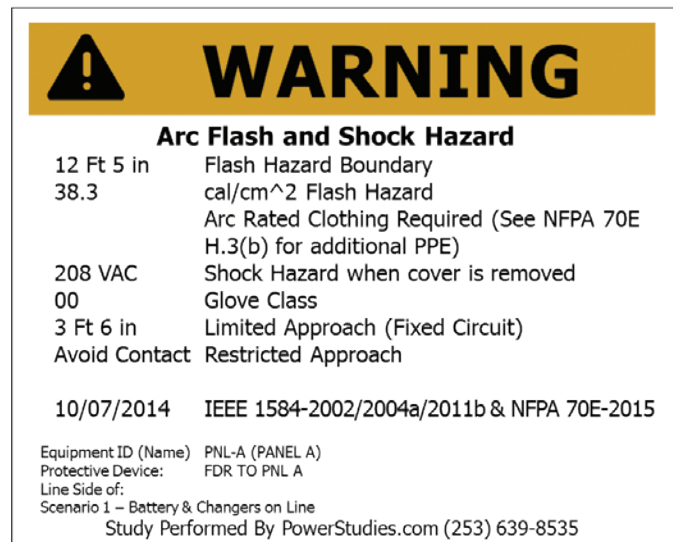
Figure 1. Example of Arc Flash Warning Label
