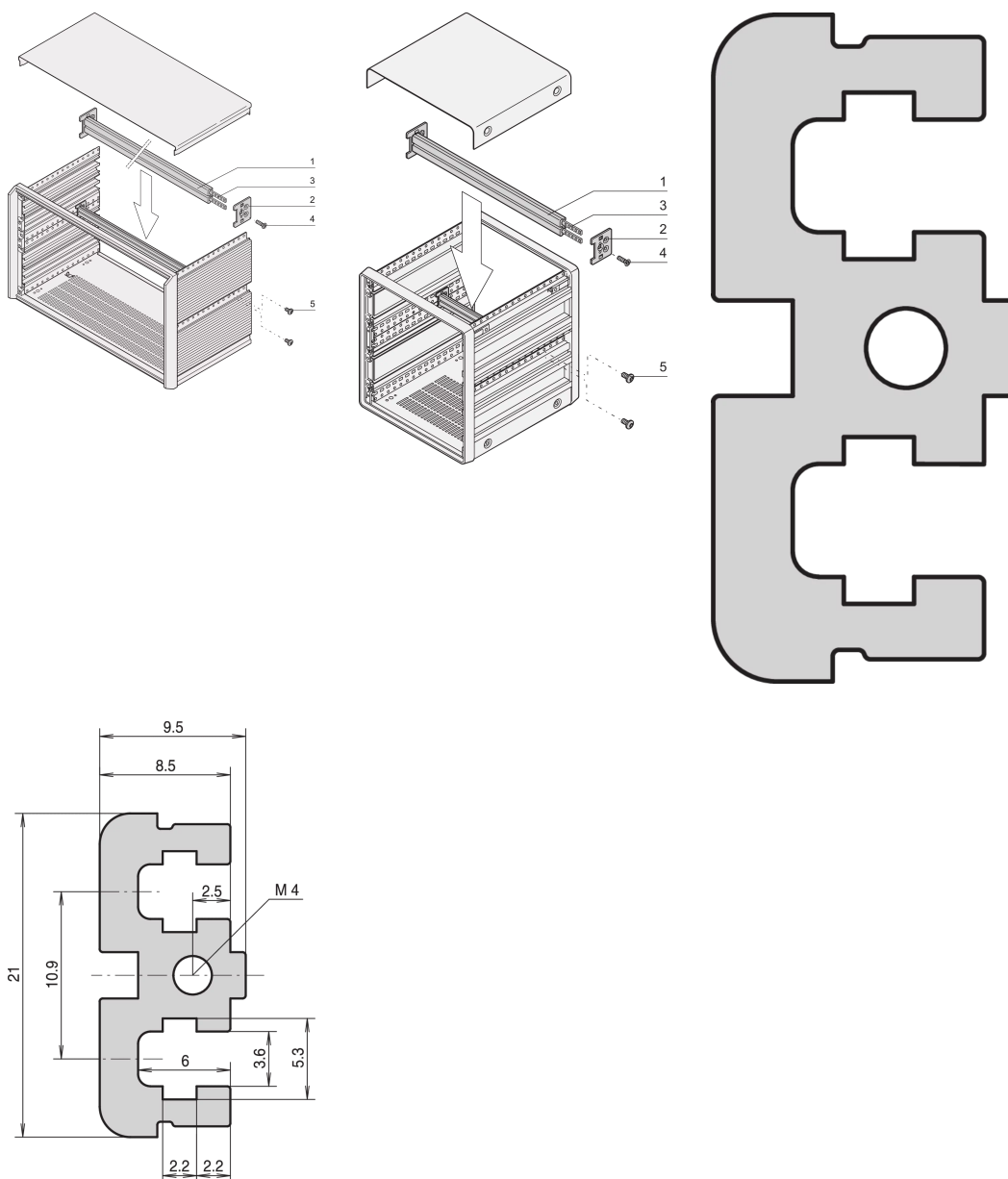
Horizontal rail, centre, type ST-C.
