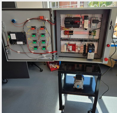
The students showcase their final working enclosure as part of the program.
