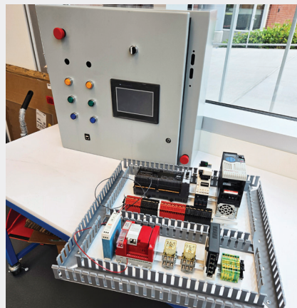
Students install and assemble all electrical components.
