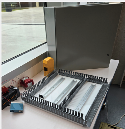
Students mount DIN Rail and Wire Duct on the back panel.
