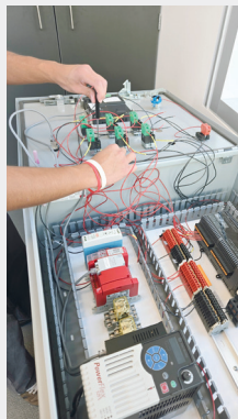
Students interact with all components making electrical connections and testing.
