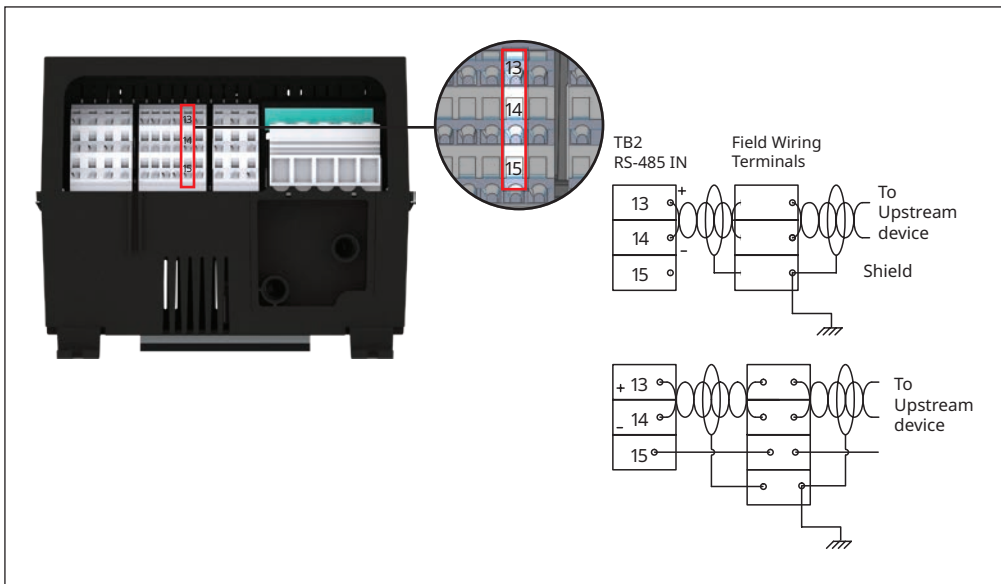
Figure 8 - RS-485 IN
