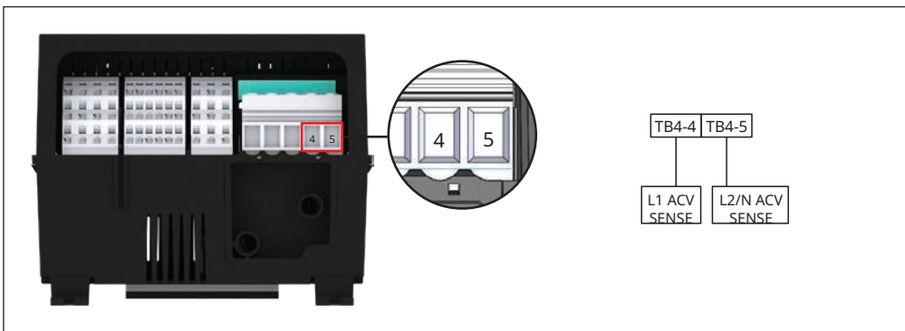
Figure 7 – Elexant 4020i - AC Voltage Sense
