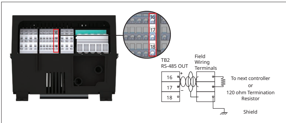
Figure 9 - RS-485 Out
