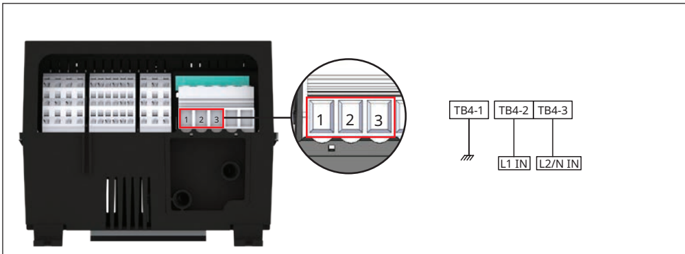
Figure 5 - Input Power
