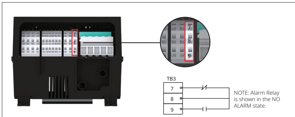
Figure 21 - Alarm Relay
