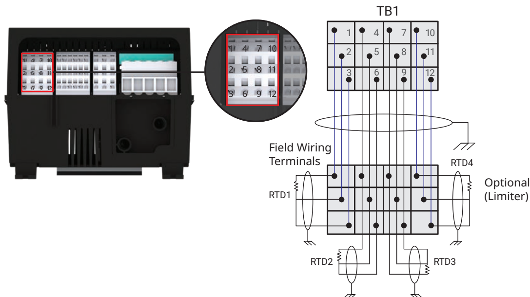
Figure 14 - 3-wire RTD connections
