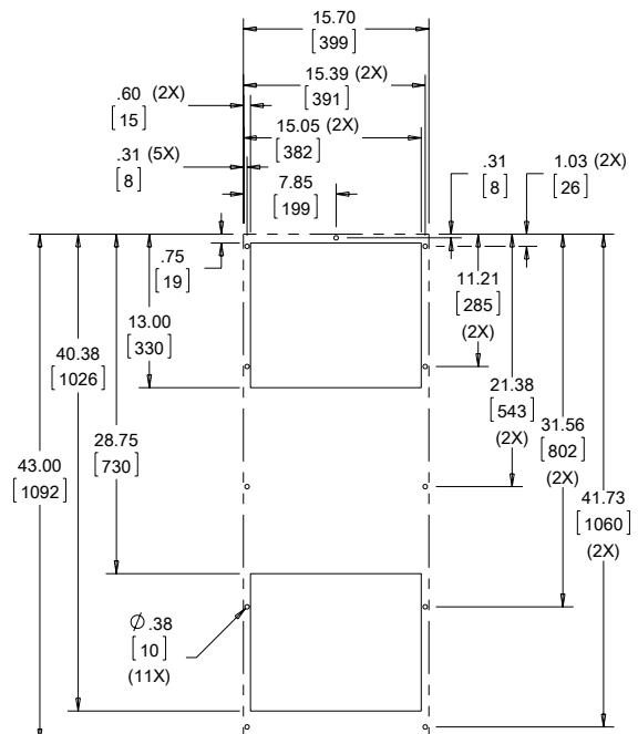
AC OUTLINE Cutout Dimensions (Externally Mounted)
