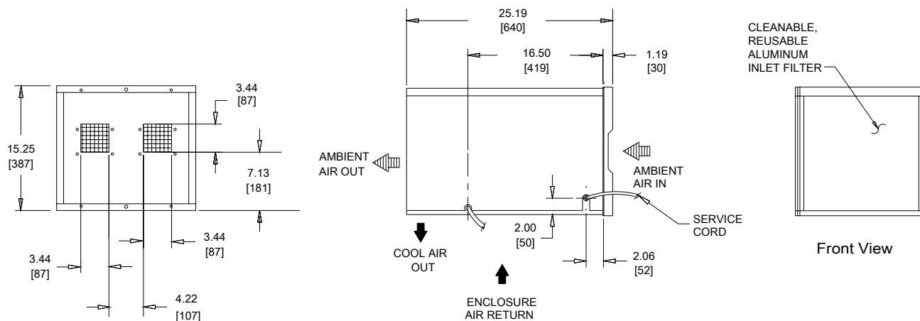
Rear View
