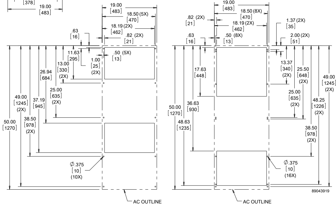
Cutout Dimensions (Externally Mounted)
