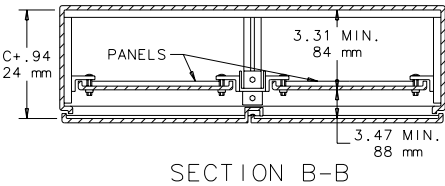
Showing two panels (for one-door enclosures) and center panel support mounted in two-door enclosure.
