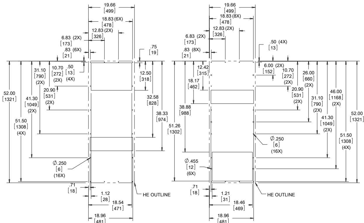
Cutout Dimensions (External Mount)
