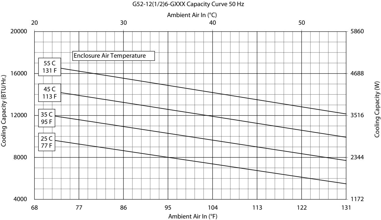
Performance Curves for G52 Models 12000 BTU/Hr. (3500 Watt)
