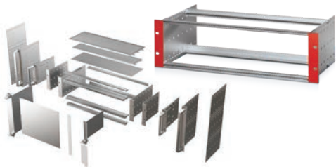
19" subracks as reliable and proven platform for modular systems solutions.
