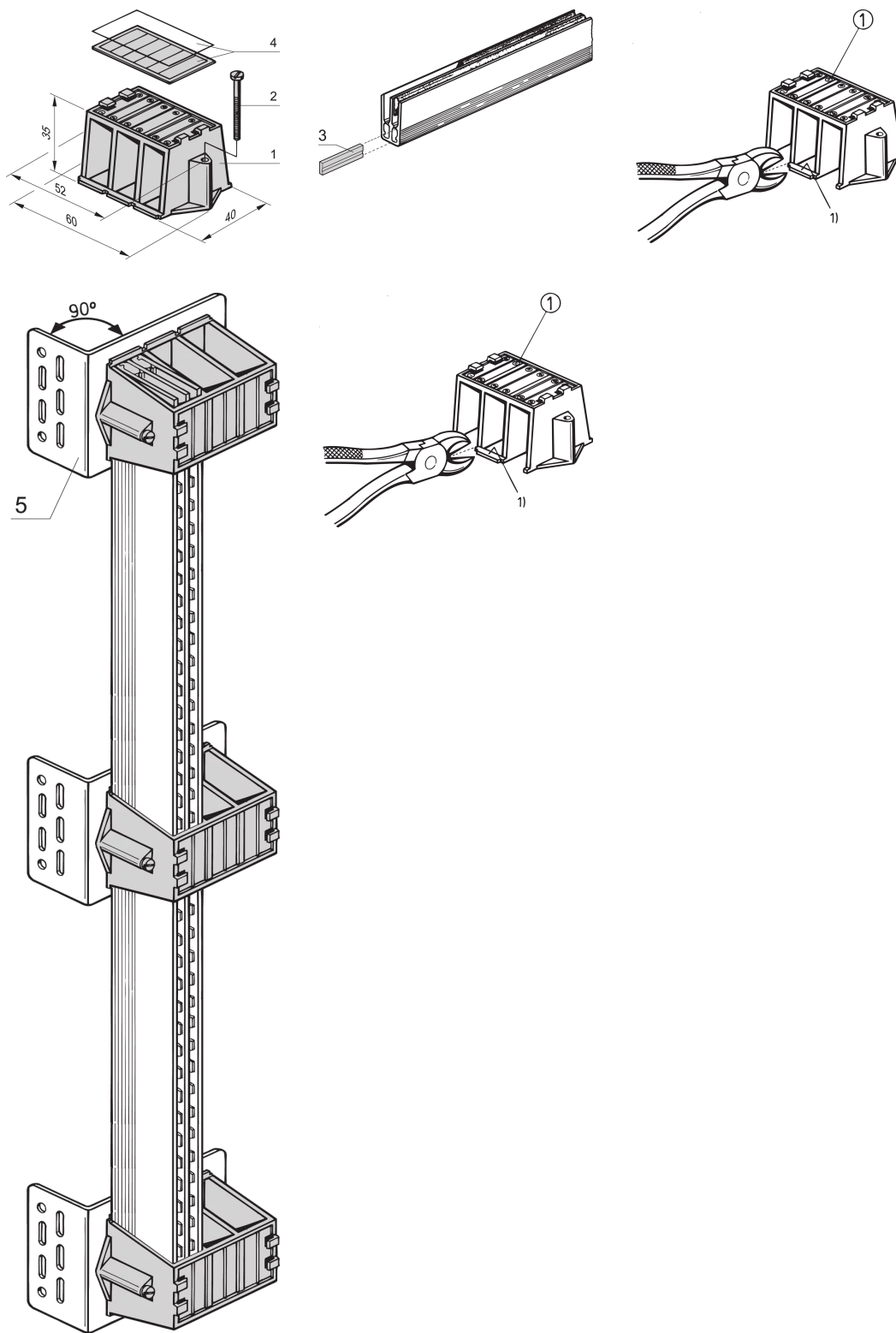
Mounting Bracket for Busbar 1, 2-Pole.
