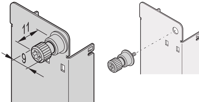
Retention Screw for MTCA.4 Front Panel.
