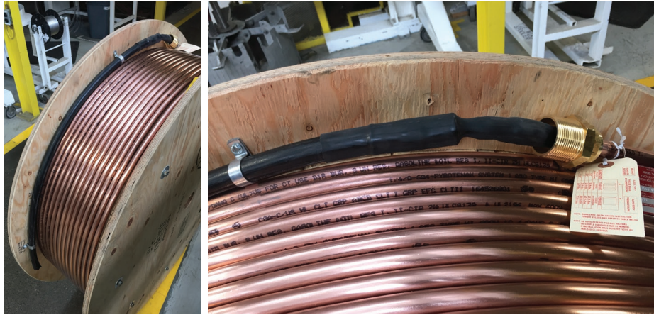
Pre-terminated 4/0 MI cable sized-up to 500 kcmil THHN tail
