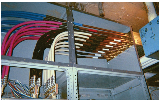
Completed MI cable termination - inside view
