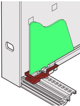
Guide rail accessories and PCB-Board- Retainer
