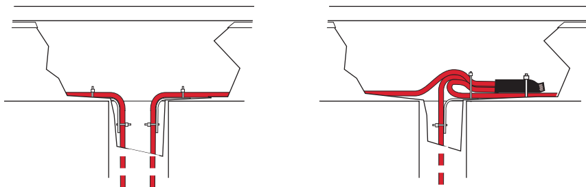
Fig. 24 GM-RAKE downspout hangers
