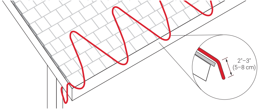
Fig. 10 Layout for heated drip loops
